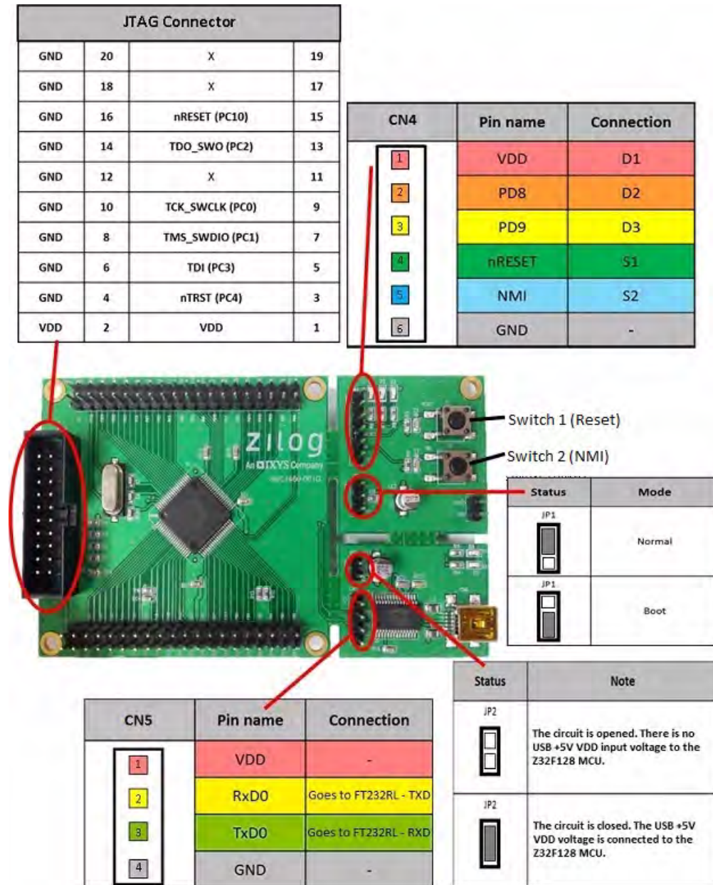
Figure 4. Jumper Settings
