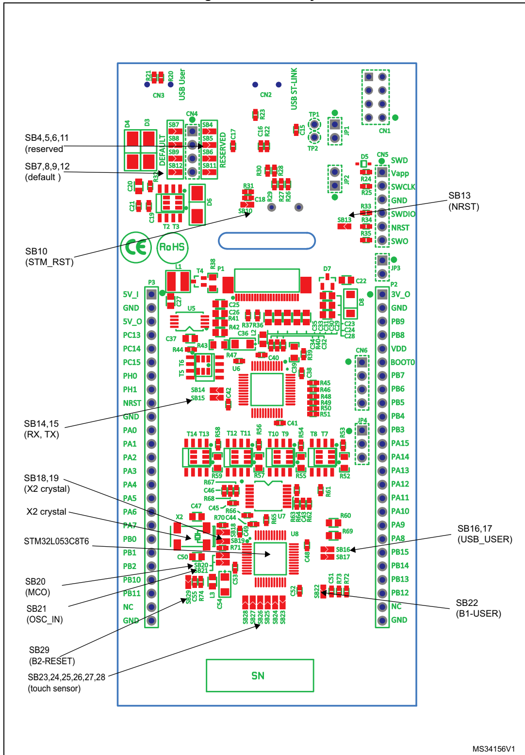
Figure 4. Bottom layout
