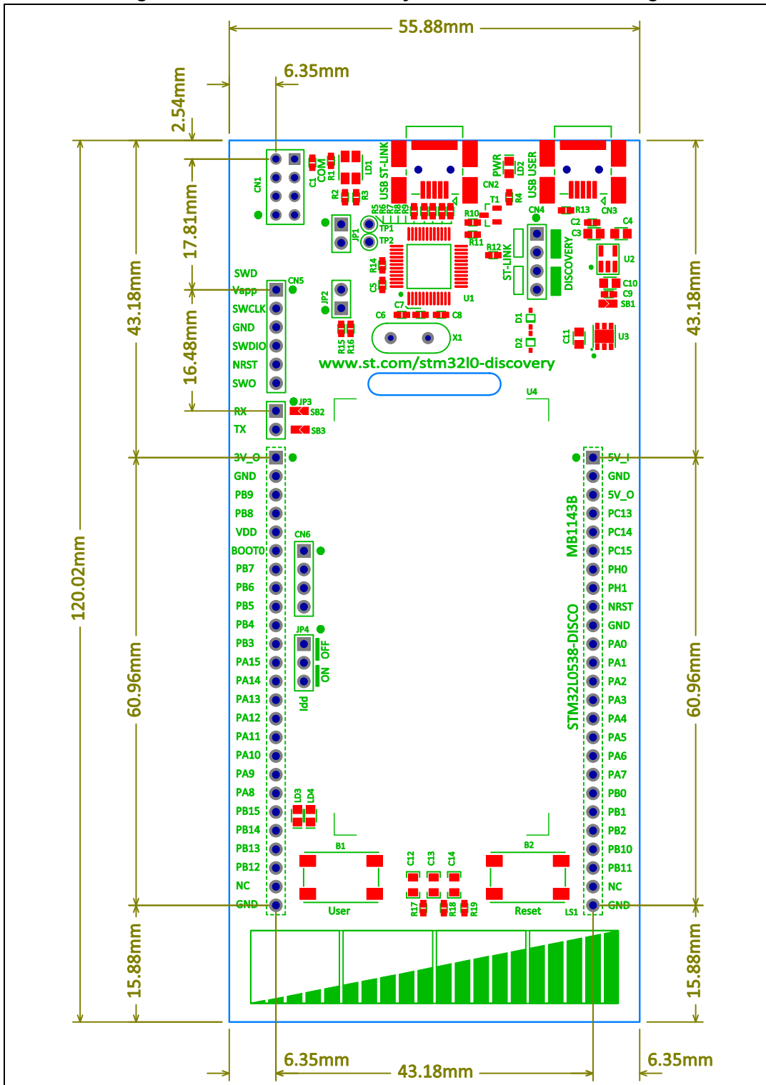
Figure 12. STM32L053 discovery board mechanical drawing
