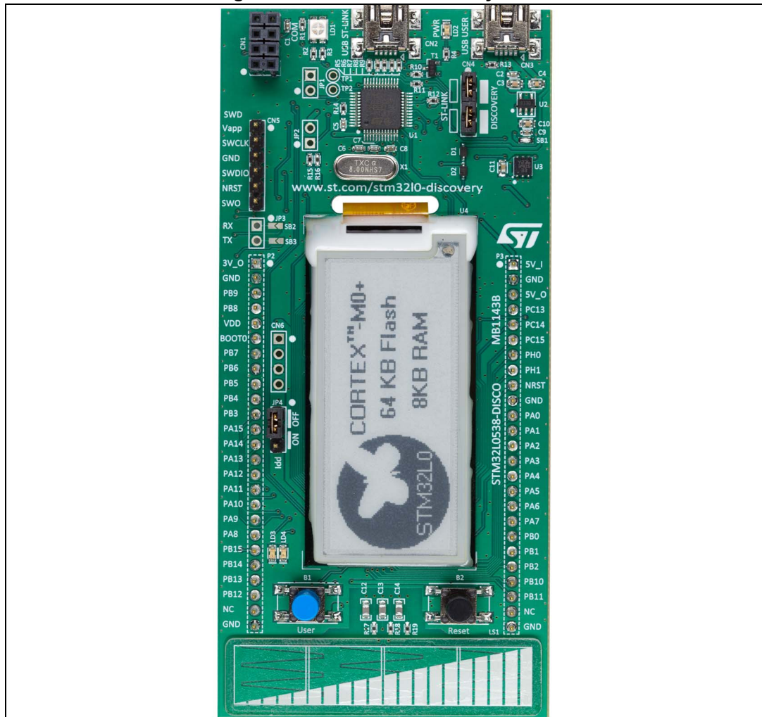
Figure 1. STM32L053 discovery board
