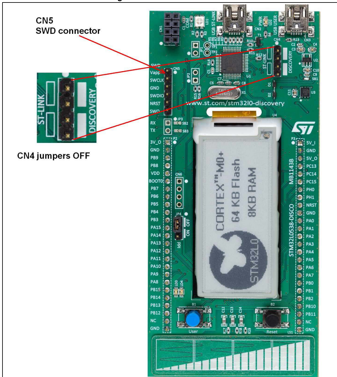
Figure 7. ST-LINK connections
