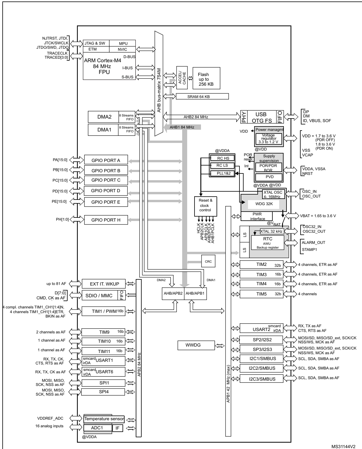
Figure 5. STM32F401VCT6 block diagram
