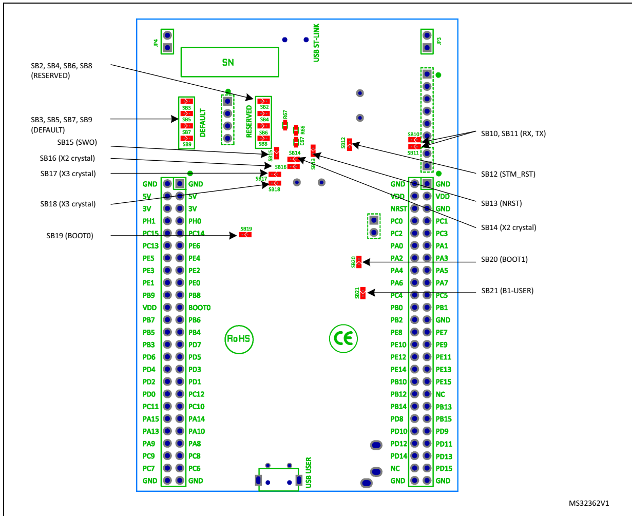
Figure 3. Bottom layout
