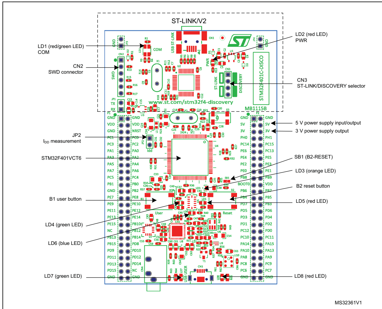
Figure 2. Top layout
