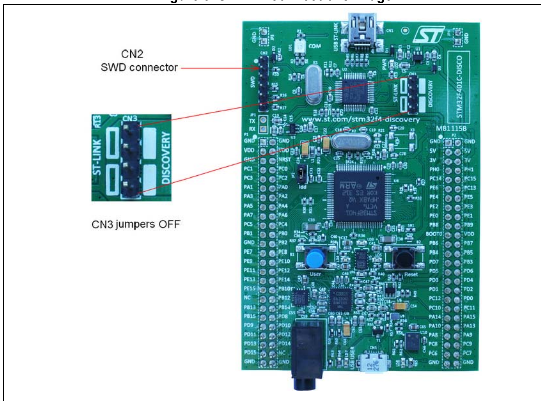
Figure 8. ST-Link connections image
